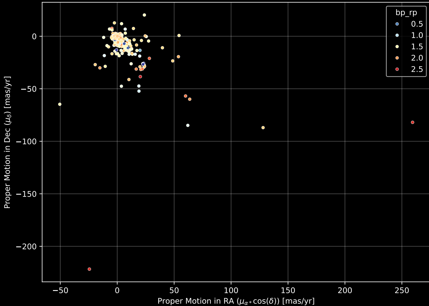
APOGEE DR17 Field: [150-08] Proper Motion Diagram (n= 564)
