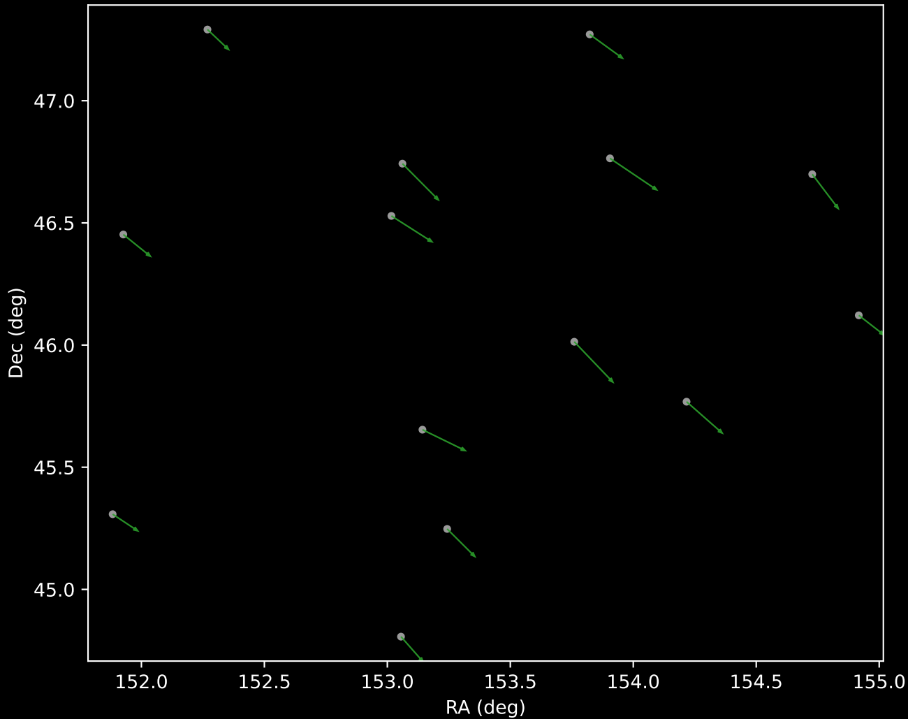
APOGEE DR17 Cluster 24 Proper Motion Vectors (n=14)
