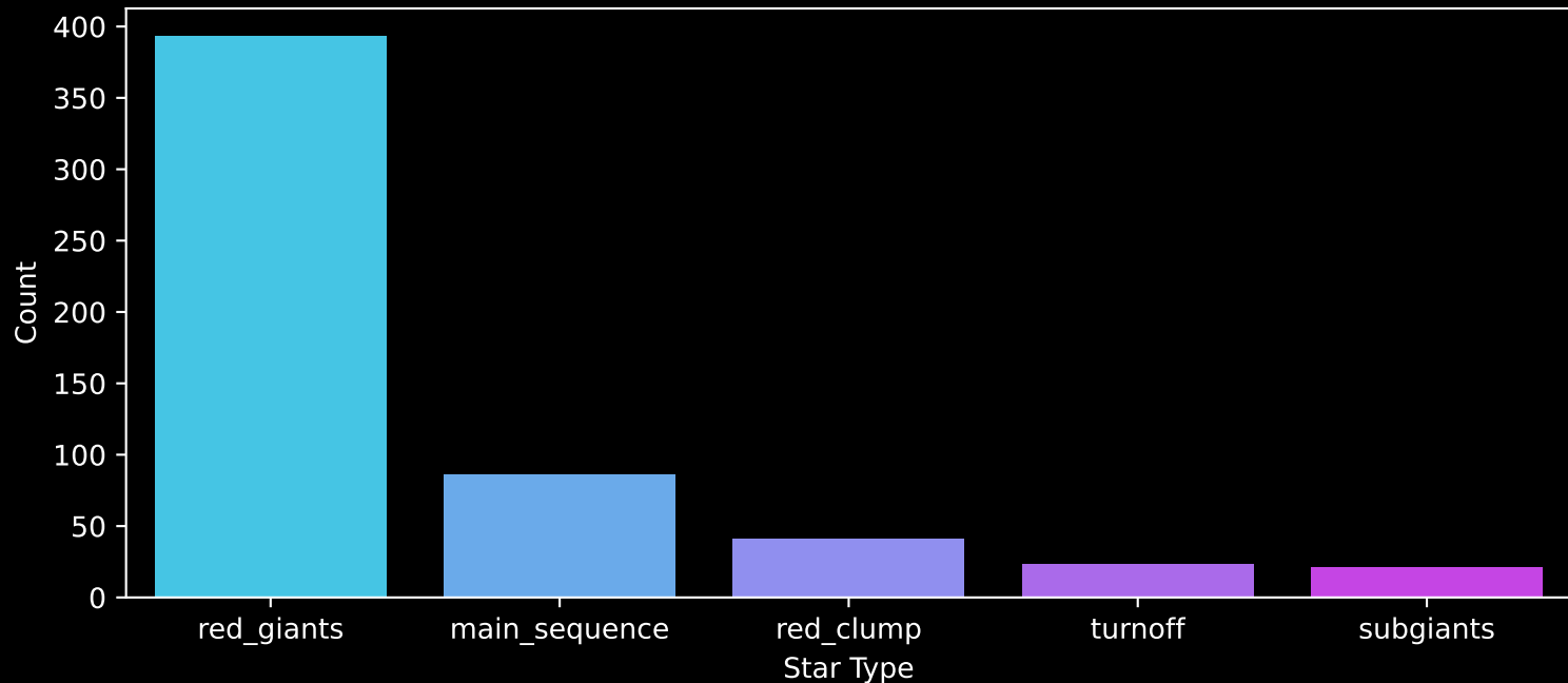
APOGEE DR17 Field: [150-08] Count plot of Star Type
