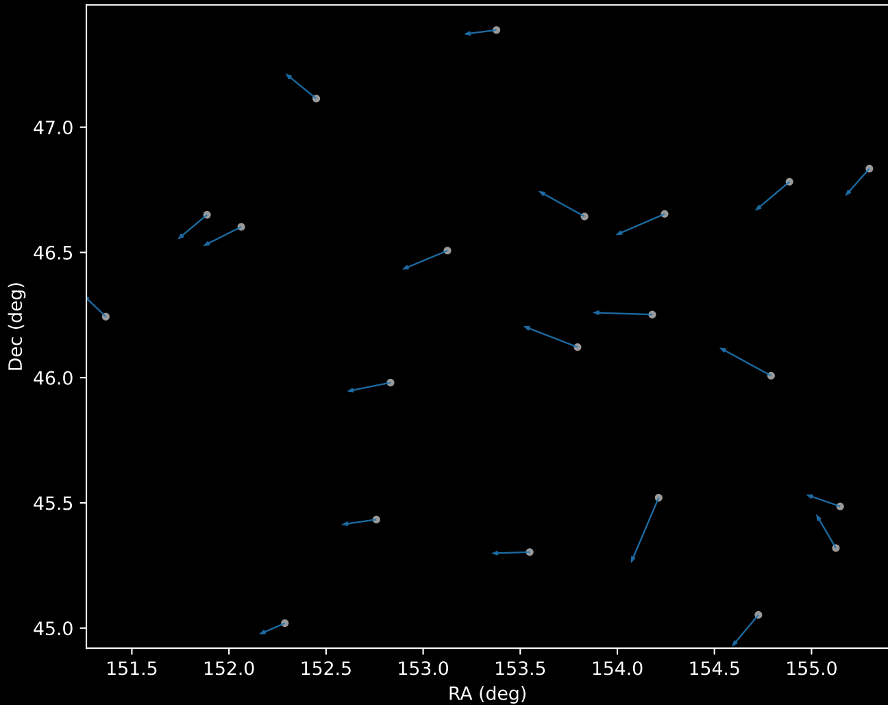
APOGEE DR17 Cluster 20 Proper Motion Vectors (n=21)
