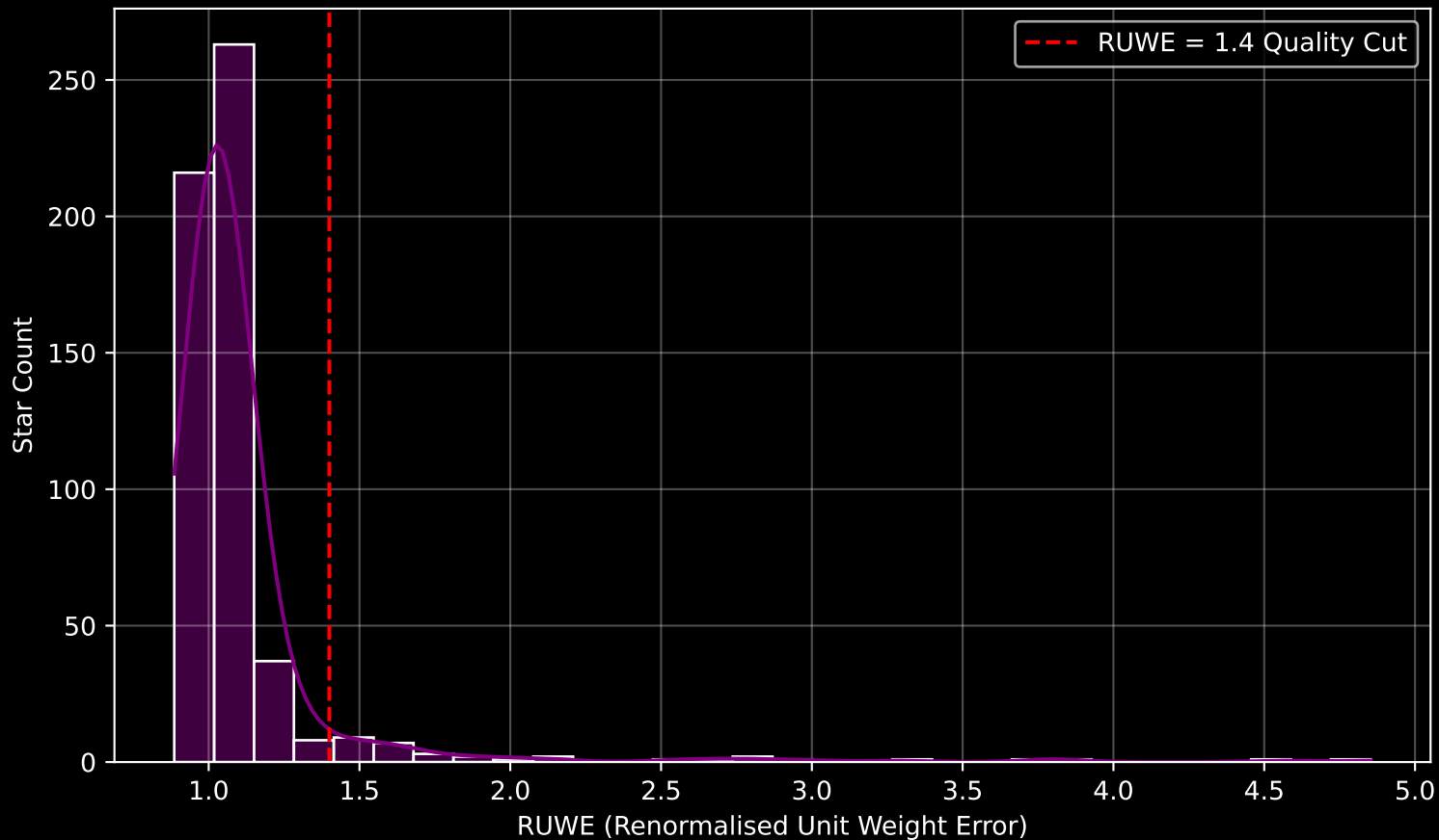
GAPOGEE DR17 Field [150-08] RUWE Distribution (n= 558)
