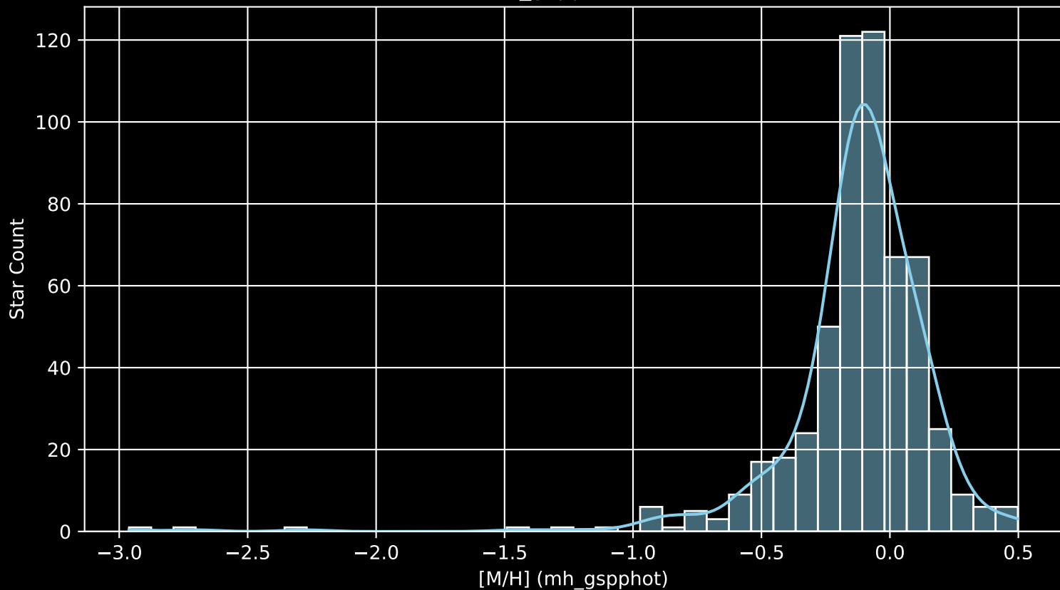
APOGEE DR17 Field: [150-08 [M/H] (mh_gspphot) (n= 562)
