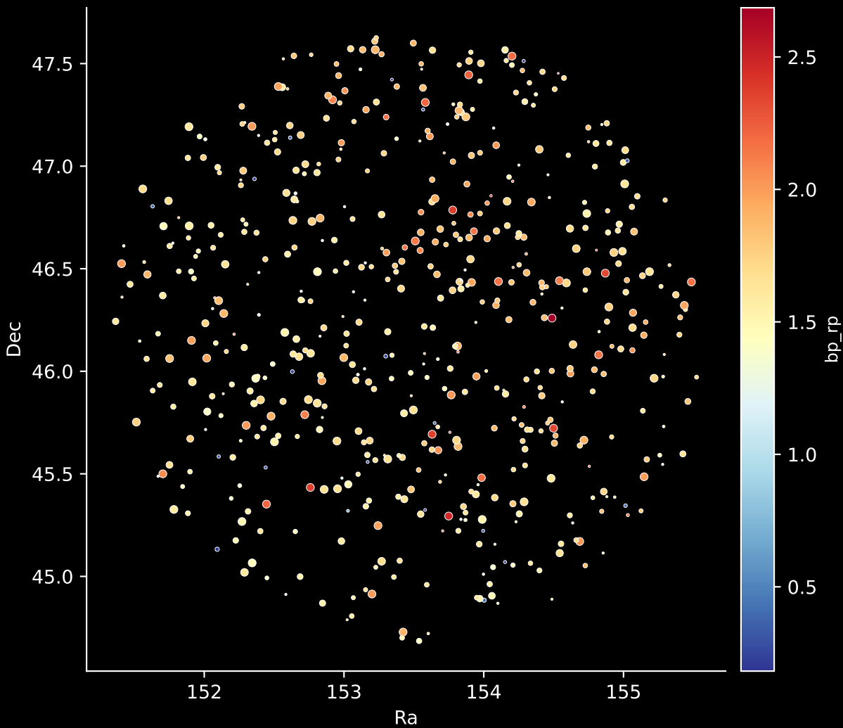
APOGEE DR17 Field: [150-08] Stars: 564
