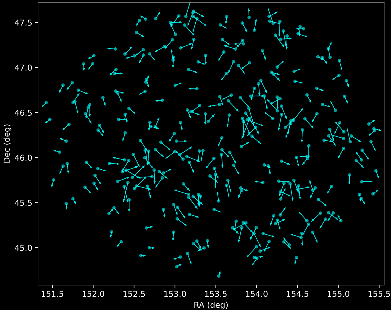
APOGEE DR17 Noise Stream Proper Motion Vectors (n=304)
