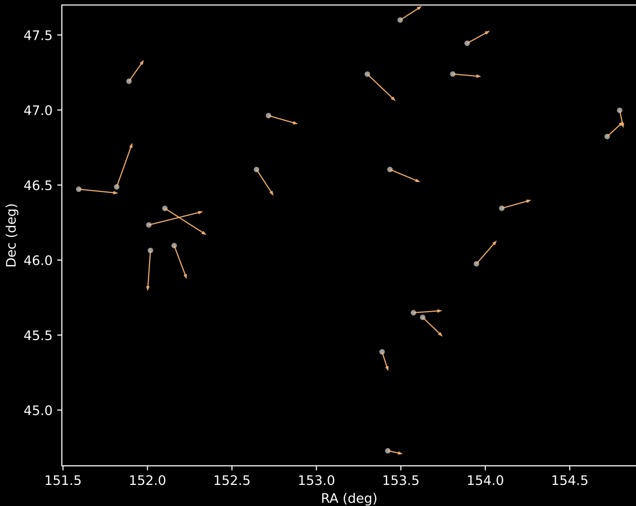
APOGEE DR17 Cluster 23 Proper Motion Vectors (n=22)
