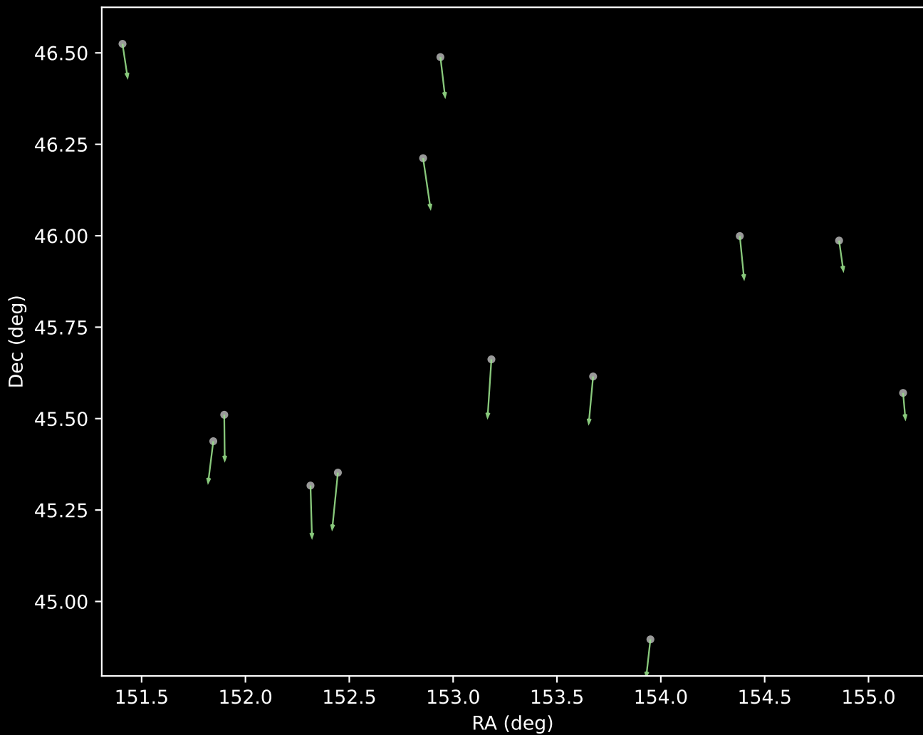
APOGEE DR17 Cluster 25 Proper Motion Vectors (n=13)
