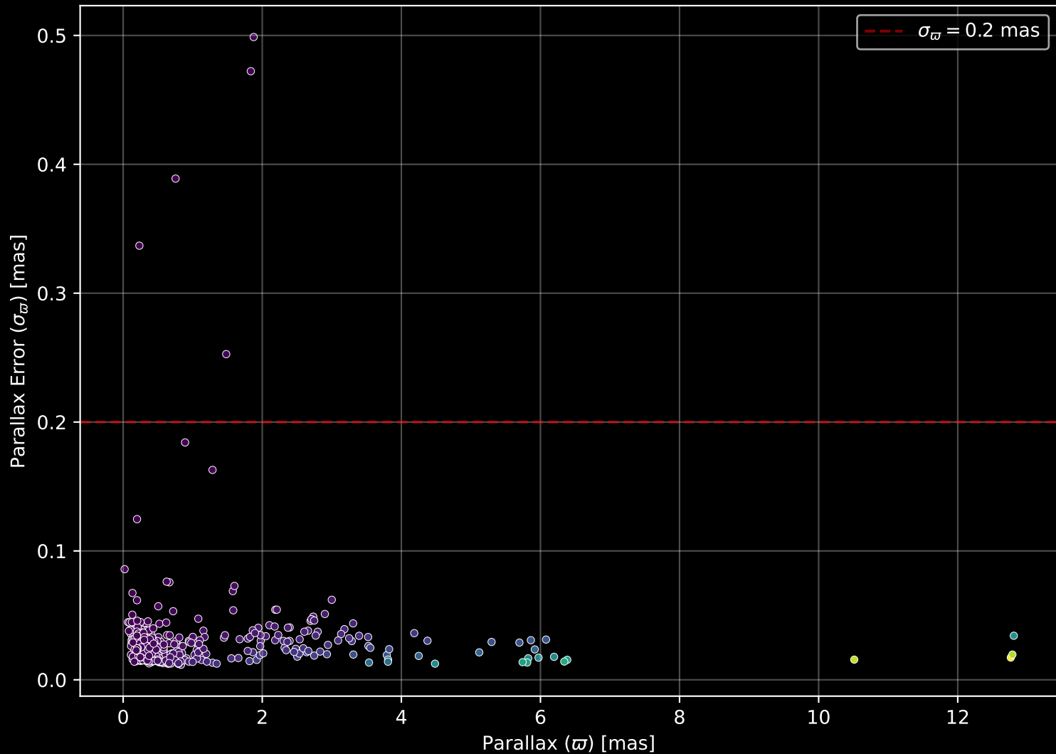
APOGEE DR17 Field: [150-08] Parallax Quality (n= 564)
